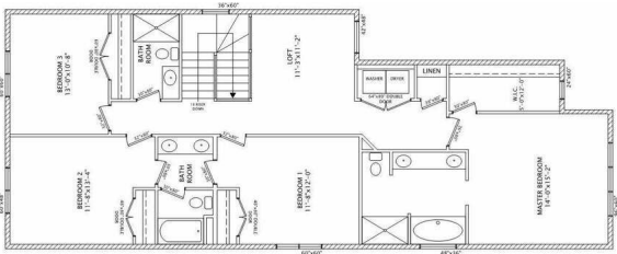
1 SECOND FLOOR PLAN
