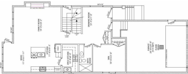
1 MAIN FLOOR PLAN
